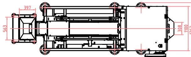
outline diagram of 6SXZ-60KI3
