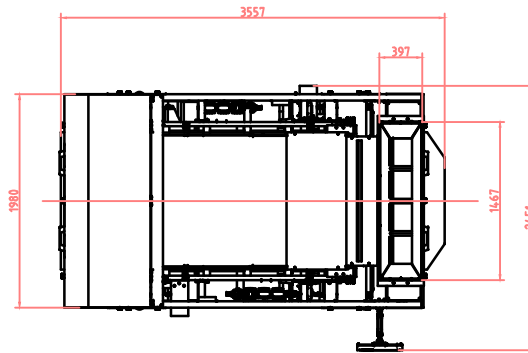
outline diagram of 480KS4
